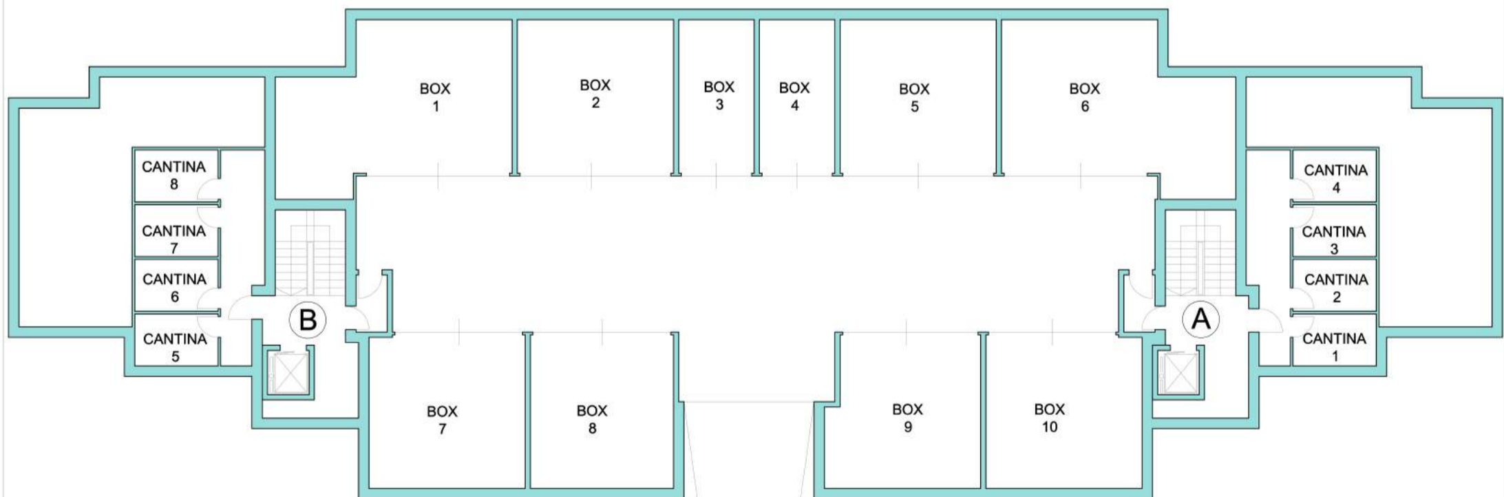
PIANO INTERRATO 1:200
