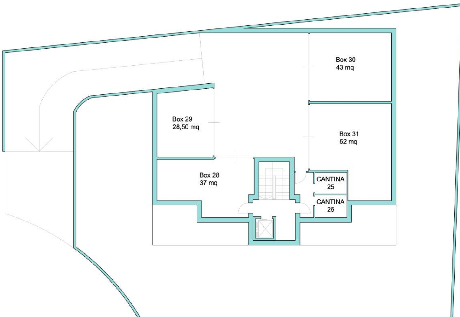
PIANO INTERRATO 1:200
